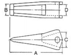
Type 1- Centerline Ripper Tooth
