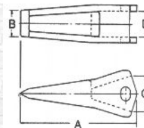
Type 1- Centerline Ripper Tooth
