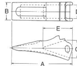
Type 3- Ripper Tooth
