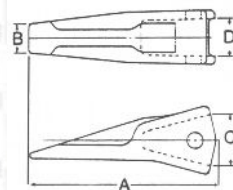
Type 2- Penetration Ripper Tooth
