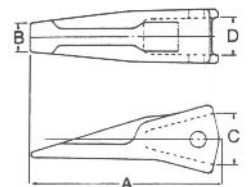
Type 2- Penetration Ripper Tooth
